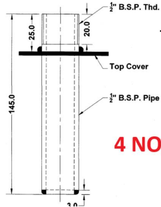
ROLLER PAD BUSH
